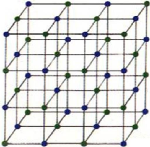
Crystalline three-dimensional-lattice-structure
